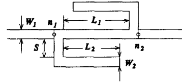
Fig. 6. Double folded stub filter.
